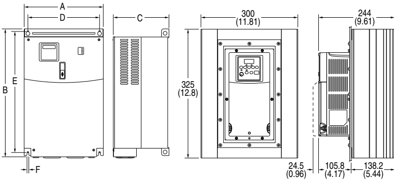
Figure 5: PowerFlex 400 Frames C-F
